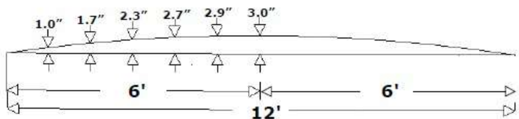
CROSS SECTION DETAIL
