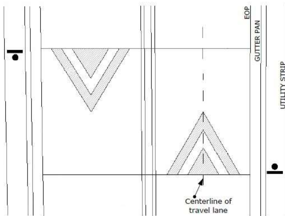
PLAN DETAIL
